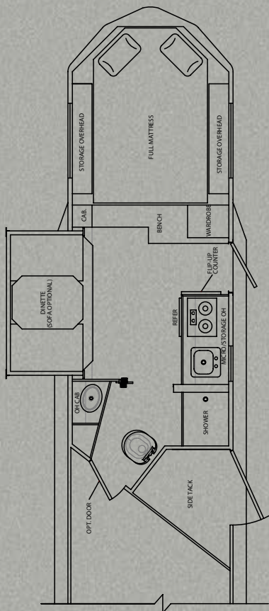
10 X 10 SIDE TACK SLIDE OUT
